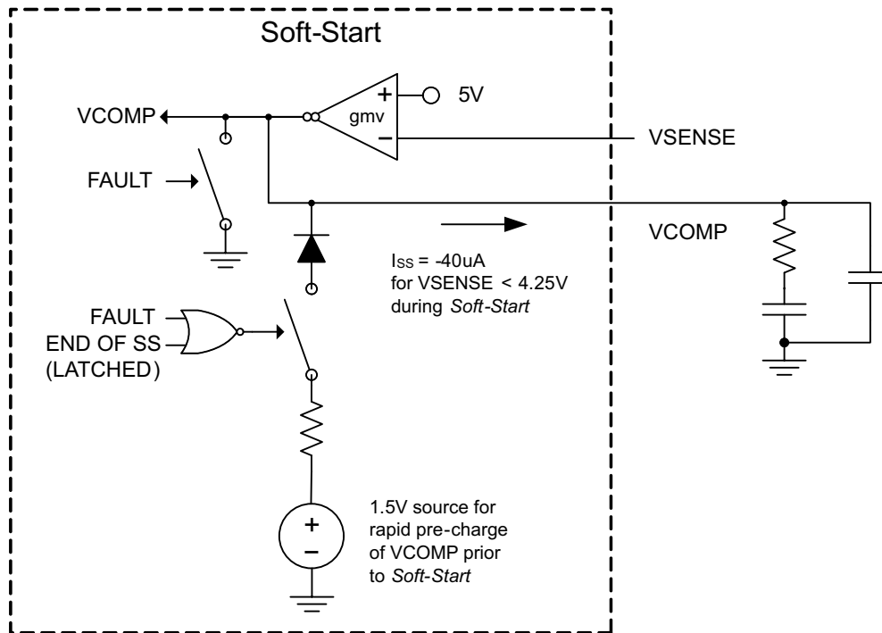
Figure 24. Soft Start
