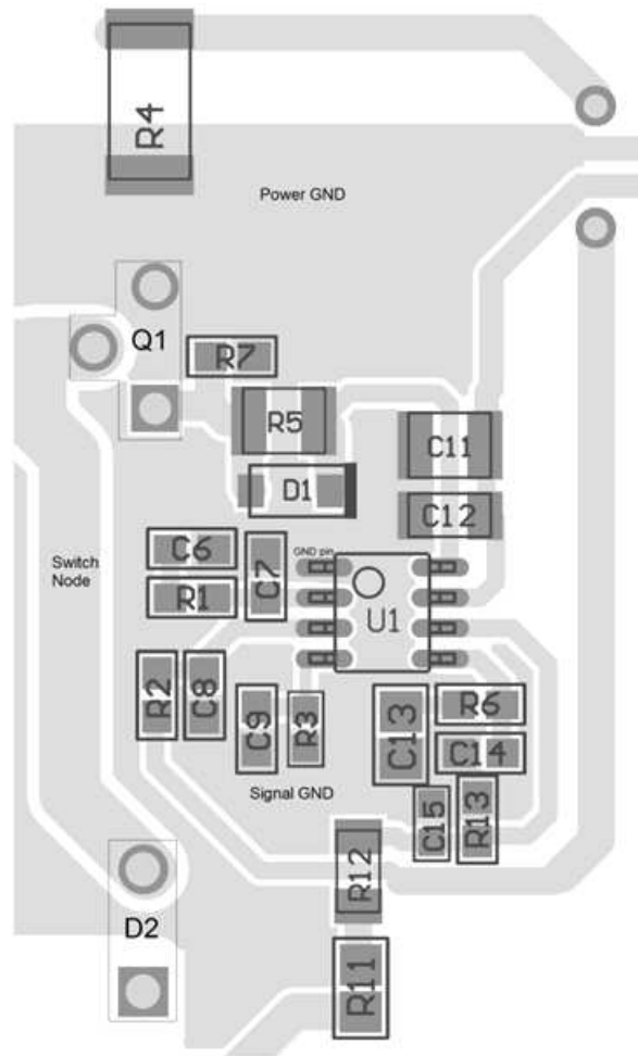
Figure 36. Recommended Layout for UCC28180
