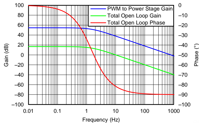
Figure 34. Bode Plot of the Open Voltage Loop without Error Amplifier
