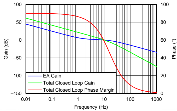
Figure 35. Closed Loop Voltage Bode Plot
