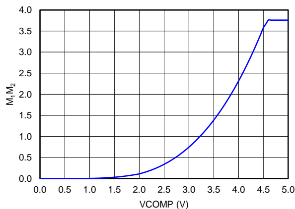
Figure 32. M1M2 vs. VCOMP
