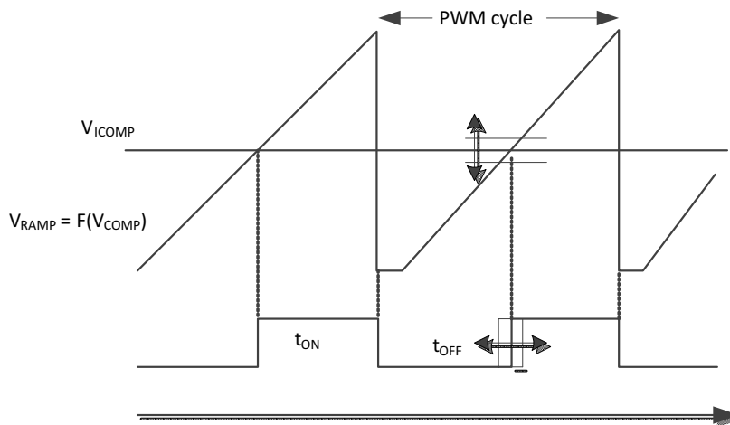
Figure 29. PWM Generation
