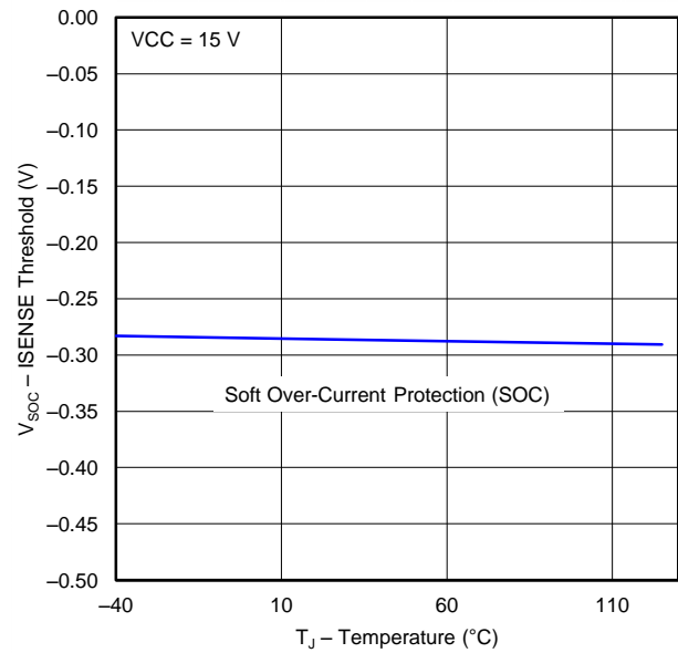
Figure 16. I SENSE Threshold Soft Over Current (SOC) vs. Temperature
