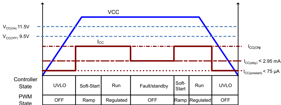
Figure 23. Device Supply States
